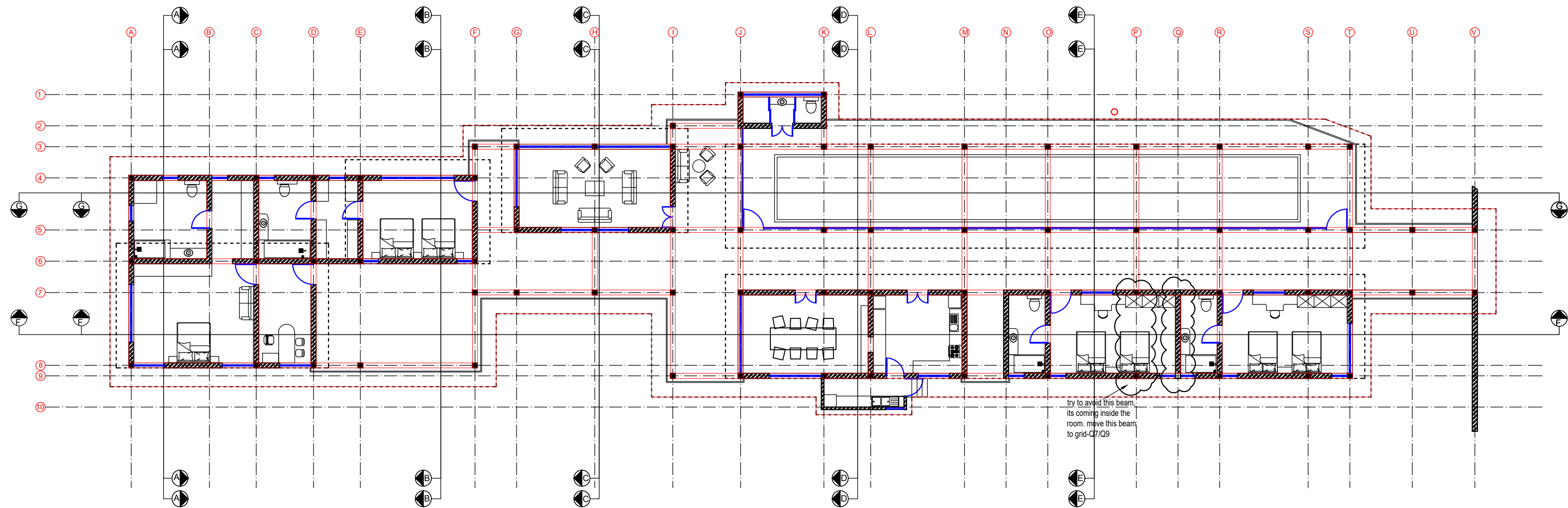
GROUND FLOOR ROOF BEAM FRAMING
